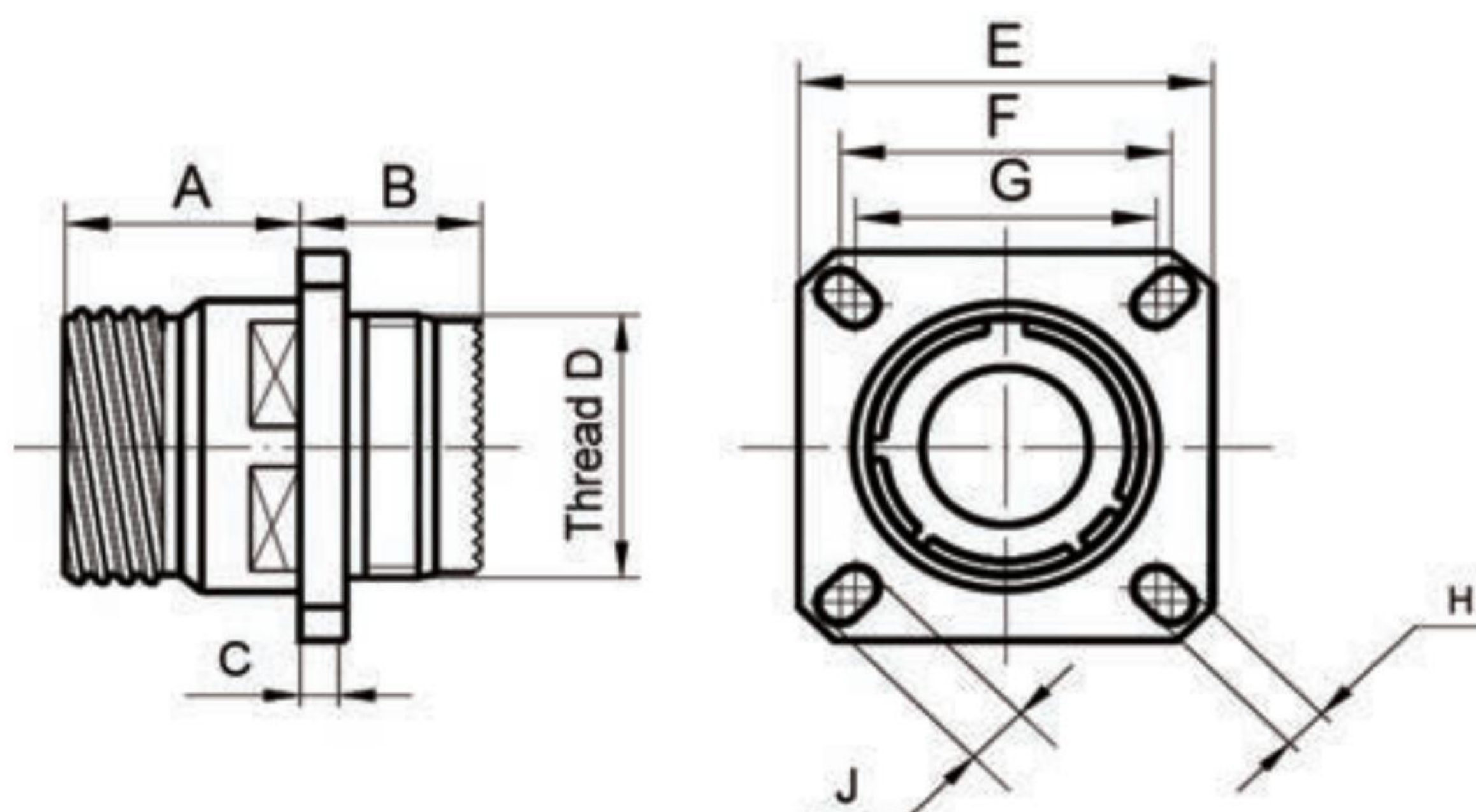
Rear Panel Mounting Hole Size
