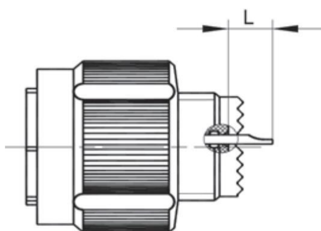
26 Type Plug
