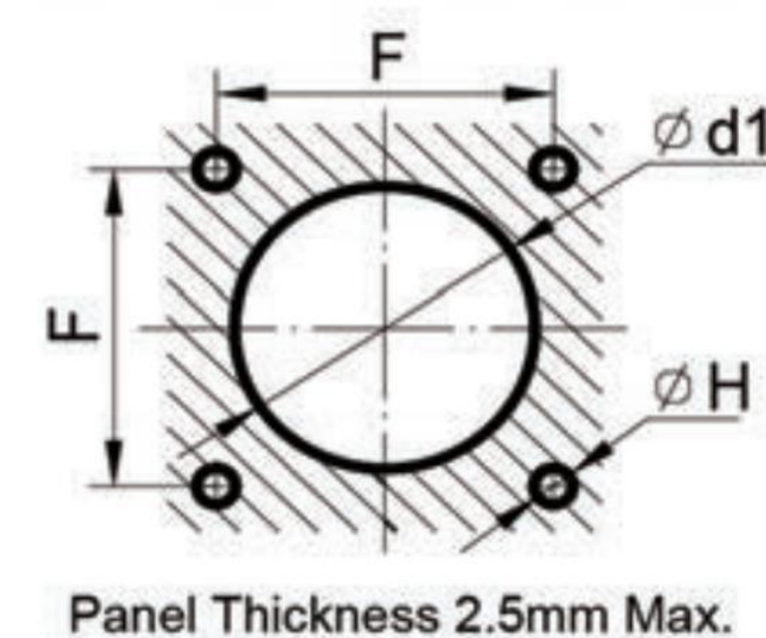
Rear Panel Mounting Hole Size
