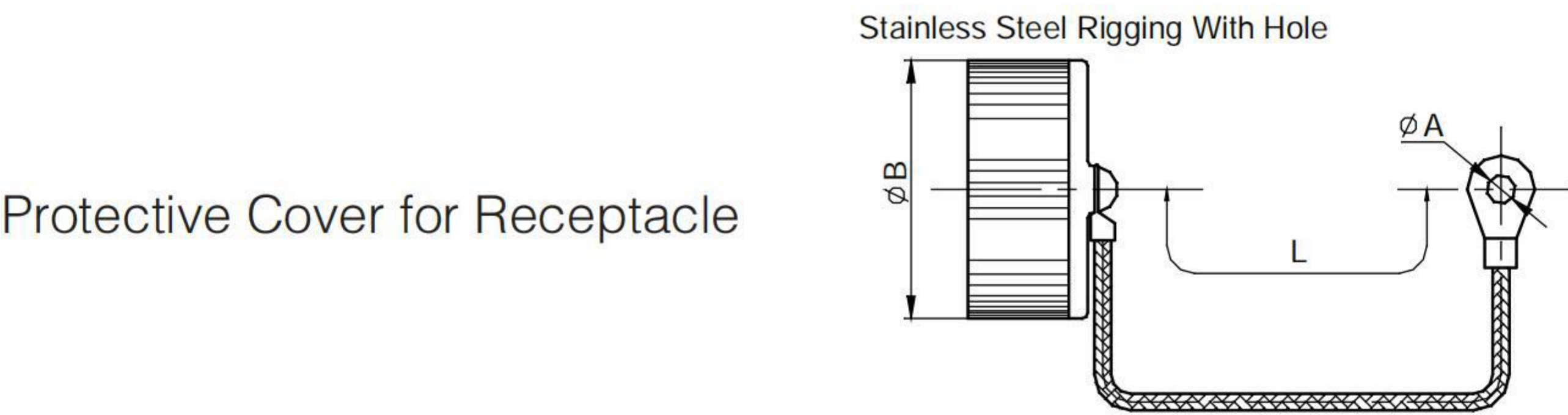
Outline Dimension
