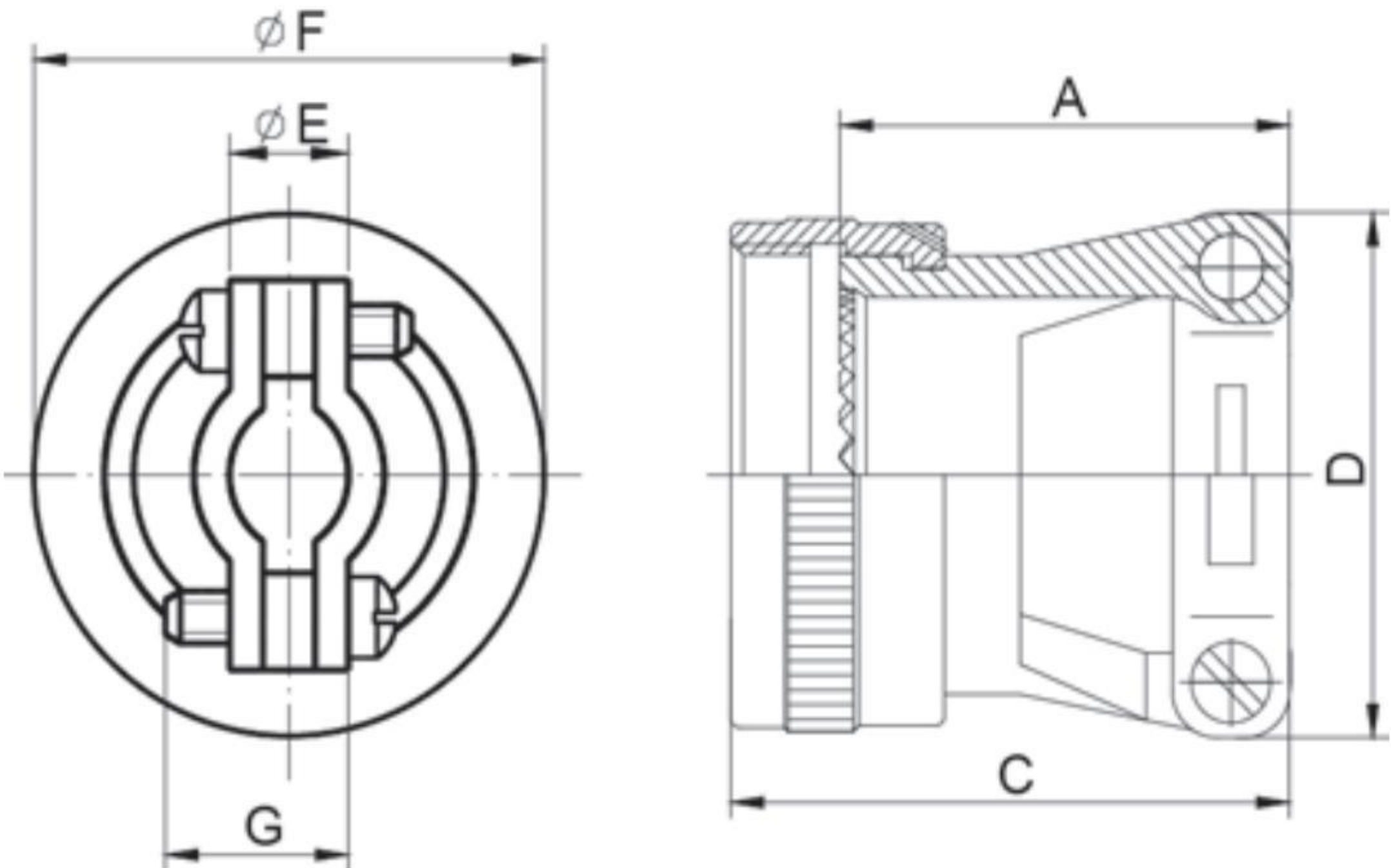
Outline Dimension
