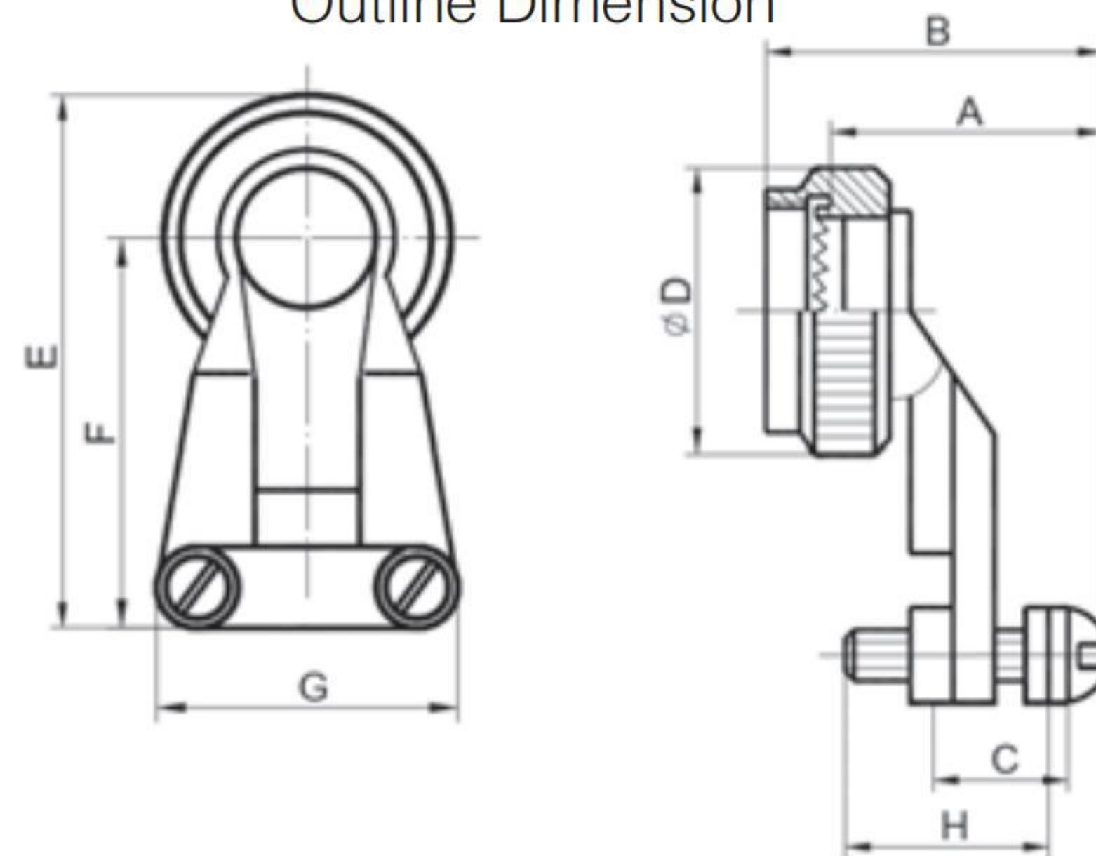
Outline Dimension
