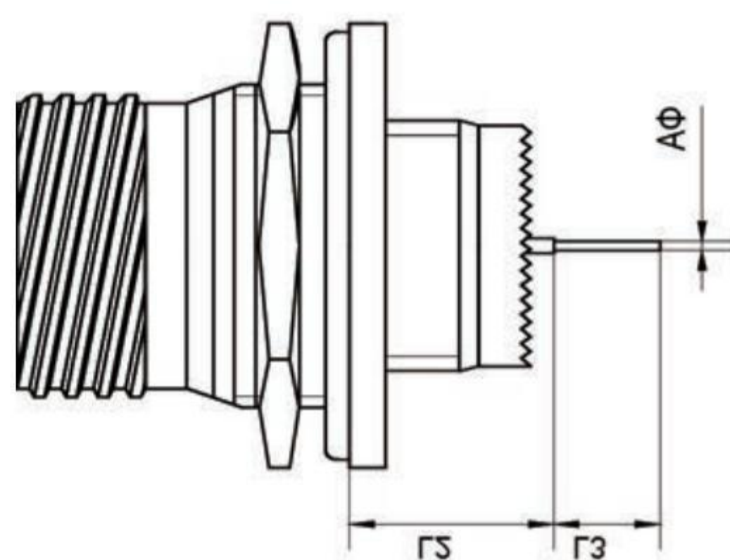
38999/24 Type Receptacle
