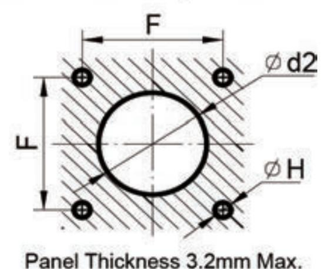
Front Panel Mounting Hole Size
