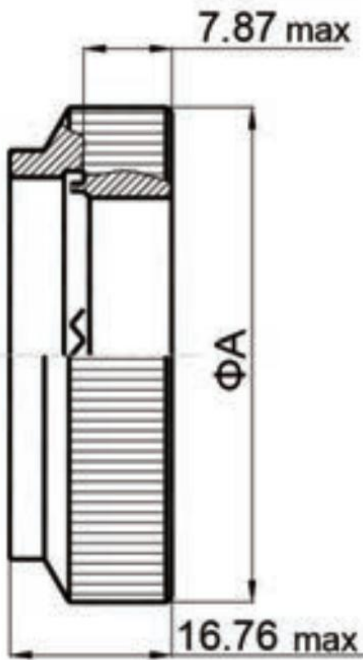
Outline Dimension
